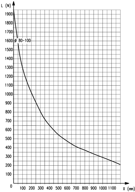
Guide "HT" moving on bush (45NHT)
