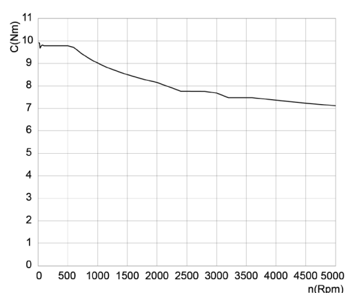
PM-6E 63... C = Torque [Nm] n = number of revolutions per minute [Rpm]
