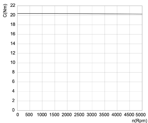
PM-6E 80... C = Torque [Nm] n = number of revolutions per minute [Rpm]
